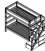
BUNK BED WITH STEPLADDER H 177 x W 257 x D 102/132 Ground clearance below the bed 25 CM Space between the beds 104 CM
