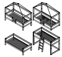
4-IN-1 CANOPY BED H128/161 x W207 x D 102/124 Ground clearance below the bed 2 / 25 / 89 CM
